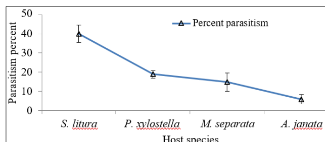
Fig 1: Host specificity of C. chloridae
